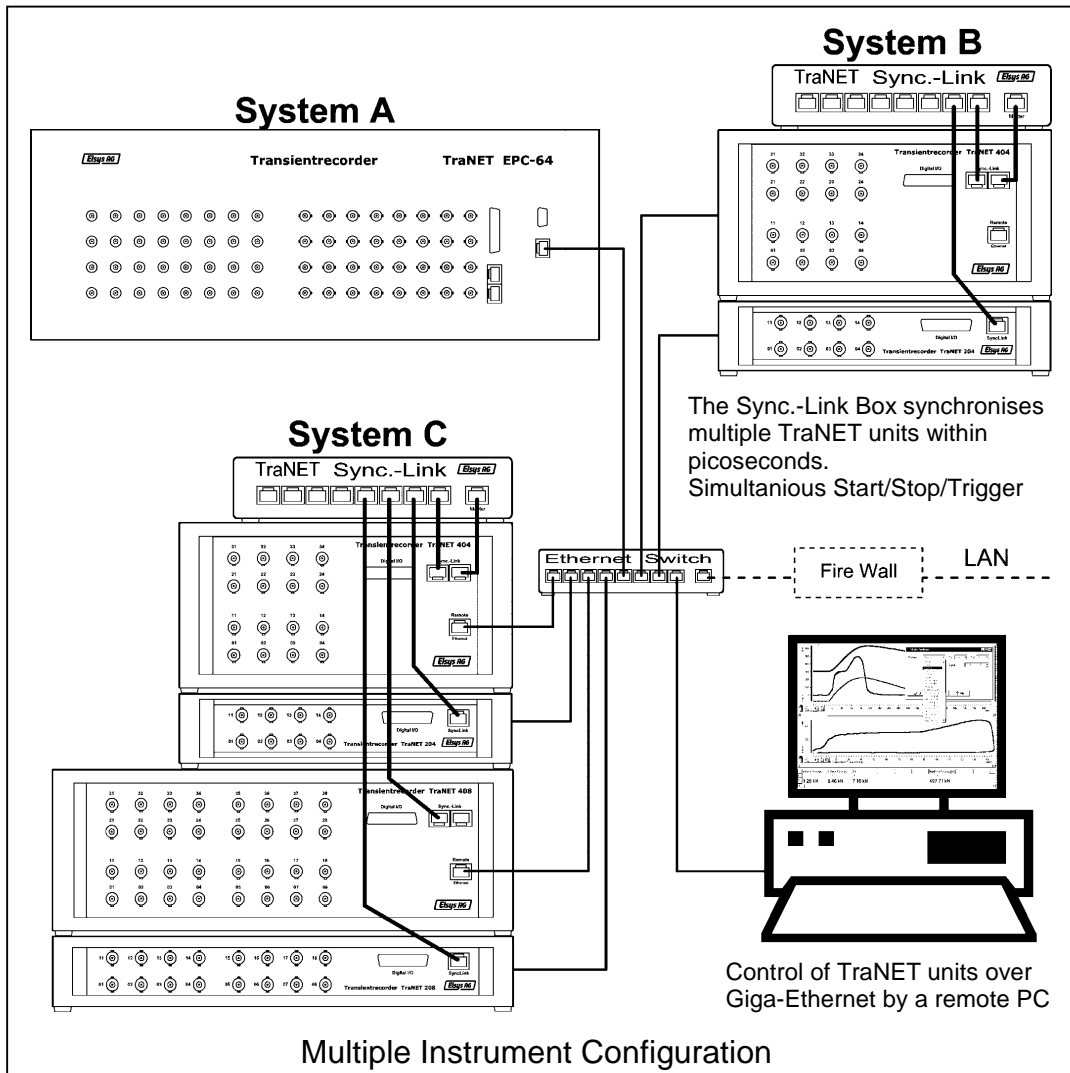
Control of several TraNET units with or without synchronisation
