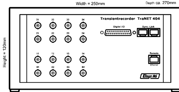
TraNET 404 4-16 Channels
