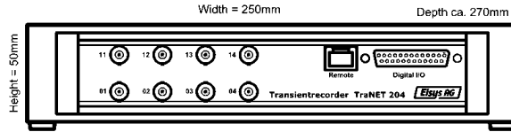
TraNET 204 4-8 Channels
